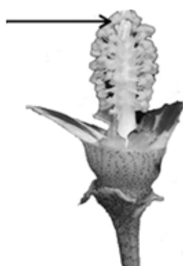
1 clearly below
