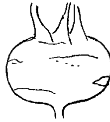
2 transverse elliptic
